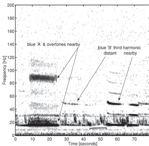
Figure 2. Spectrogram of ARP data showing blue whale A (pulsed) and B (tonal) calls, fin whale down-swept calls (~35 Hz to ~15 Hz), and ship noise (continuous tones). The B call has a series of harmonically related nearly tonal components. The B third harmonic is the detection call because of its high signal-to-noise ratio (SNR).
