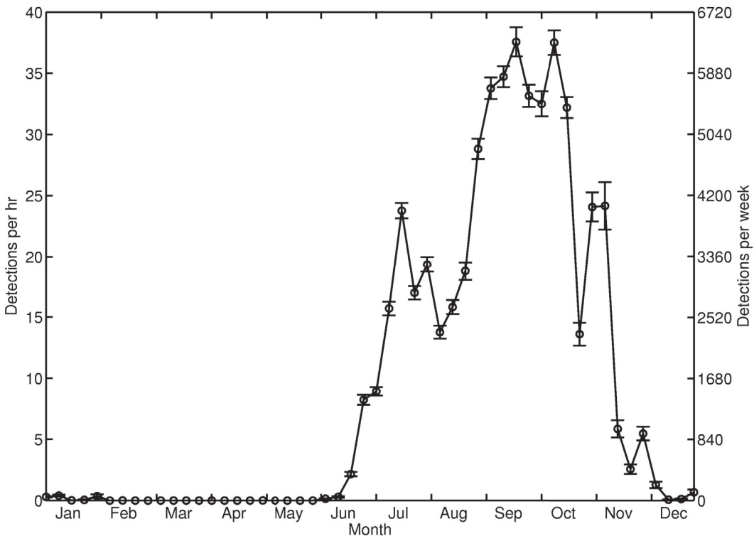
Figure 3. Number of detections/h averaged in one-week time periods and per instrument for 2001; error bars are \pm SE. The right vertical axis shows the total number of detections in the one-week time periods per instrument.
