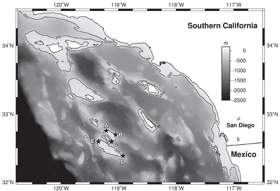
Figure 1. Southern California Bight bathymetry map with 200-m contours; the five stars depict the acoustic recording package (ARP) locations on Cortez and Tanner Banks (see Table 1).
