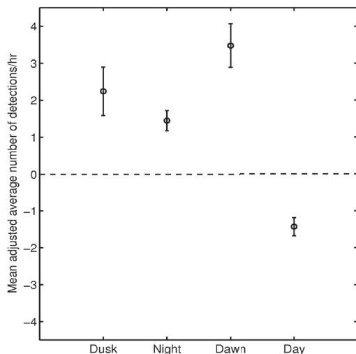
Figure 4. Adjusted average number of detections/h in four diel periods for n = 207 days; daily diel periods were obtained for 2001 at 32^{\circ} 36' N , 119^{\circ} 08' W from the U.S. Naval Observatory's Astronomical Application Department (Anonymous, 2001). Error bars are \pm SE values.
