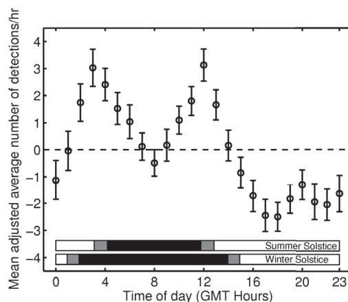
Figure 5. Adjusted average number of detections/h in GMT-based 1-h periods during 2001 ( n = 207 ; error bars are \pm SE values); horizontal bars at bottom of plot show day (white), dawn and dusk twilight (gray), and night (black) periods for the two extreme light regimes during the summer and winter solstices.
