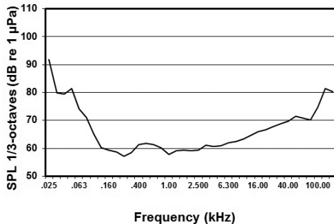
Figure 2. The background noise level in the outdoor pool during test conditions. Above 10 kHz, the noise measurements were influenced by electronic noise.
