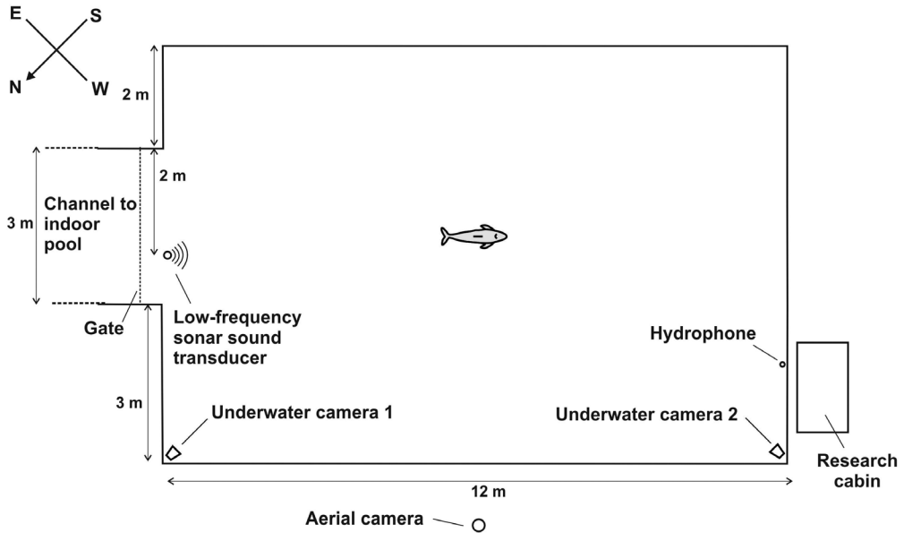
Figure 1. Top scale view of the outdoor pool at the study facility, showing the study animal, the location of the aerial camera, the two underwater cameras, the underwater transducer emitting the sonar sounds, and the listening hydrophone. Also shown is the research cabin that housed the equipment and the operator.
