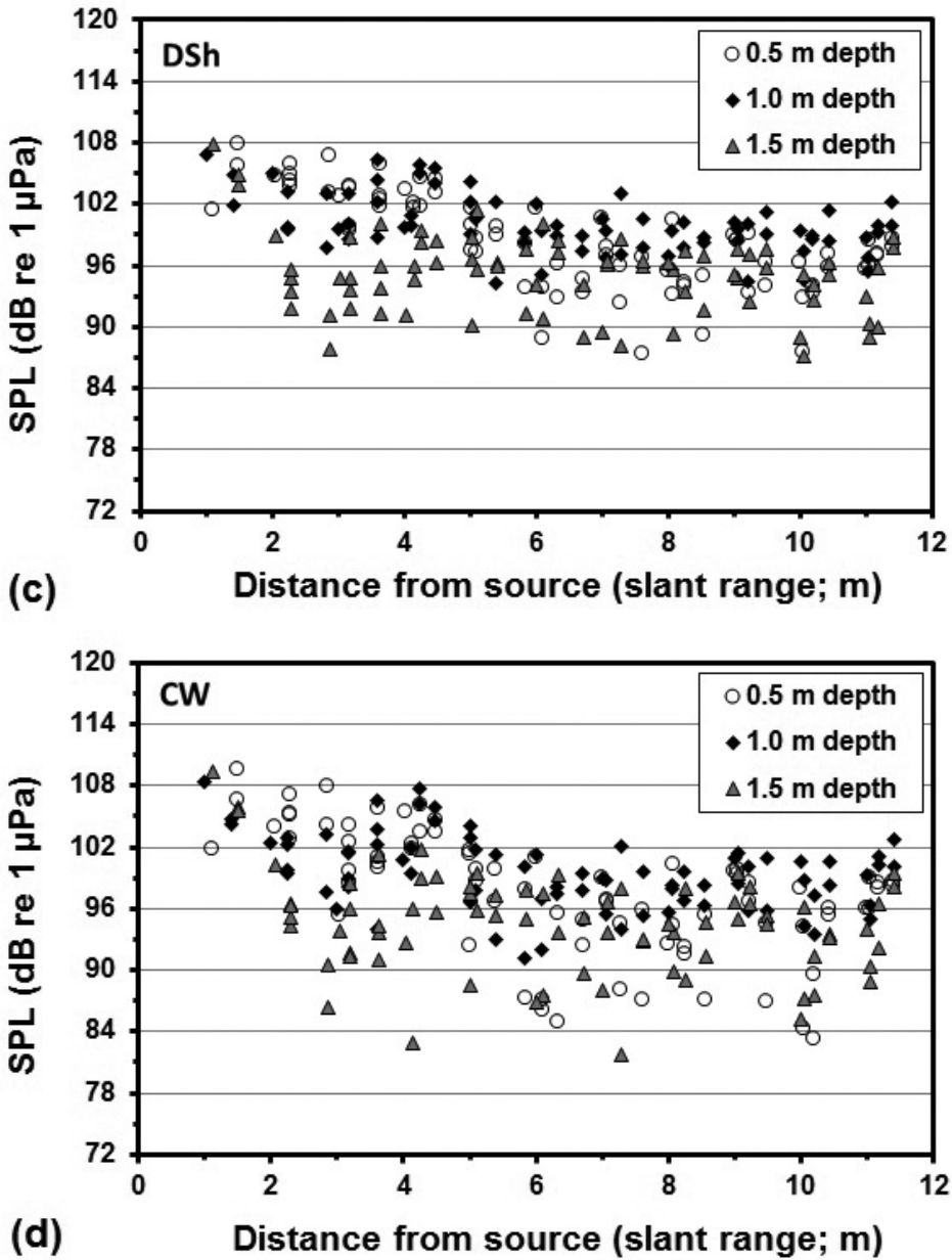
Figure 5. The SPL distribution (dB re 1 \mu Pa, averaged over the 90% energy duration of the sounds) of the four simulated sonar sounds as a function of the distance (slant range) between the transducer and the hydrophone: (a) CWht, (b) CWwh, (c) DSh, and (d) CW. As expected, the SPL range per distance is smaller for the DSh sound (c) than for the CW sounds (a, b & d).
