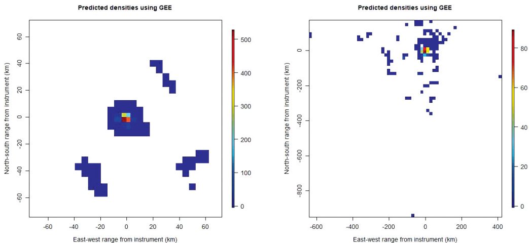
Figure 4. Two estimated georeferenced plots from the 2010/2011 season (left) and 2012/2013 season (right) showing the irregular and patchy estimated monitored area given assumptions based on measurements of SL, NL, TL, and detector performance. The colors depict the estimated call density ( \text{calls}/\text{km}^2 ). Note, however, that the apparent low density at larger ranges from the instrument may be due to overestimation of the monitored area, and, thus, these areas are omitted from the final part of the analysis.
